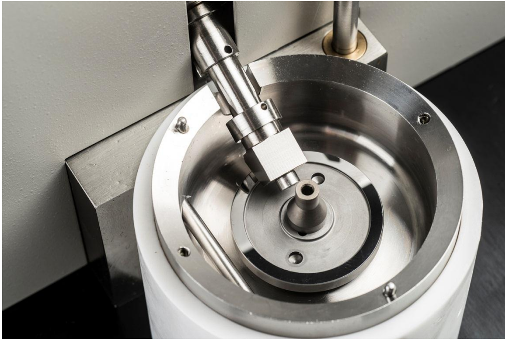
Figure 1: MTM lubricant reservoir showing pin on disc adapter.
